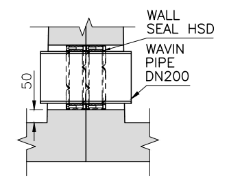
DETAIL 'C' SCALE 1:20 @ A3
