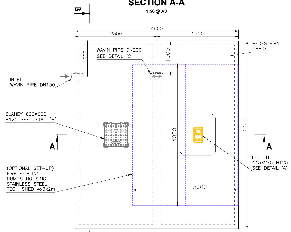
LAYOUT PLAN 1:50 @ A3
