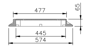
LEE FIRE HYDRANT COVER CLEAR OPENING: 445X275 CLASS B125
