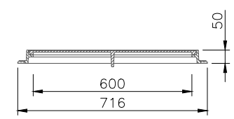
SLANEY COVER CLEAR OPENING: 600X600 CLASS B125
