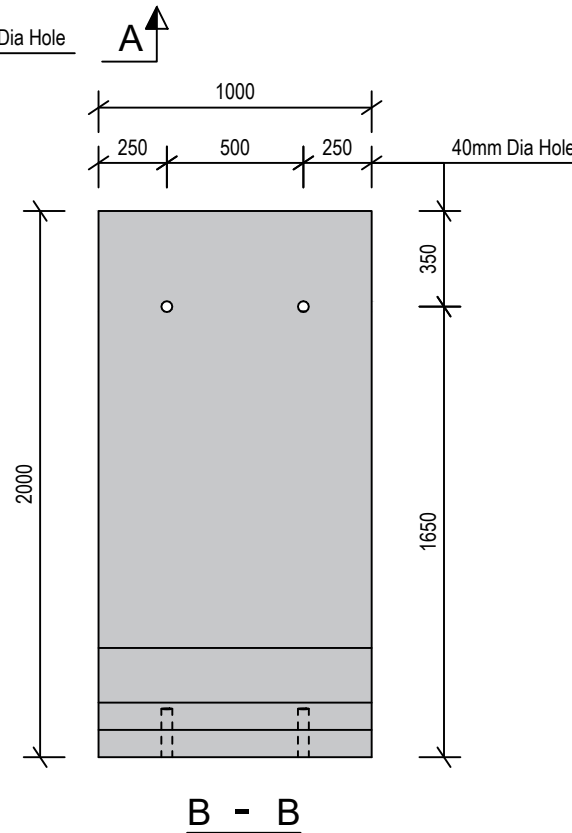
2.0 m HEIGHT L WALL
